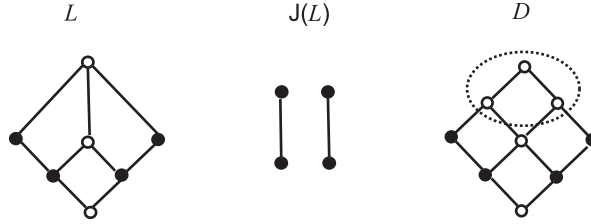
FIGURE 3. L , J(L) and the corresponding distributive lattice D = H(J(L))
