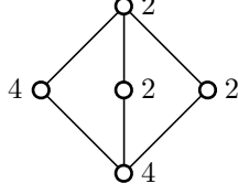
FIGURE 4. A valuation on M_3 .
