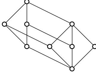
FIGURE 2. A lattice representing \langle 5, 4 \rangle .
