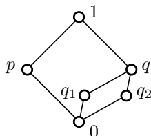
FIGURE 1. The lattices N_6 .
