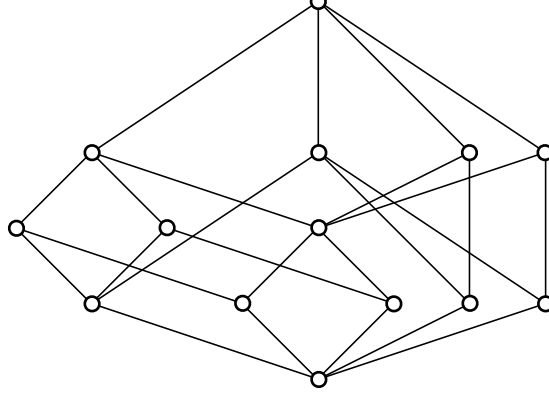
FIGURE 3. A lattice representing S = (4, 4, 2, 2, 2) .
