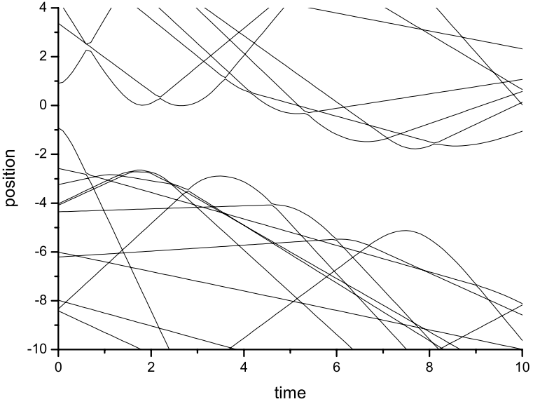
Fig. 1. Trajectory of the particles with indices |i| \leq 30 for the time interval 0 < t < 10 in the Type II dynamics, with c = 10 .
