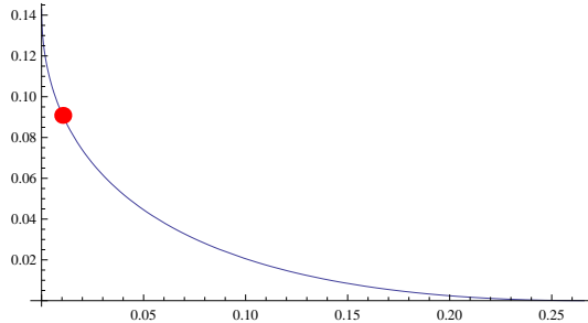
Figure 1: The macroscopic shape of the positions of q -Hahn TASEP particles for q = 0.2 , \mu = 0.4 , \nu = 0.3 which is given by the blue parametric curve (f/\kappa, 1/\kappa) . Due to the technical condition (2.16), Theorem 2.5 is valid for positions which are on the right of the red dot on the plot, i.e. for the major part of the rarefaction fan for these values of the parameters.
