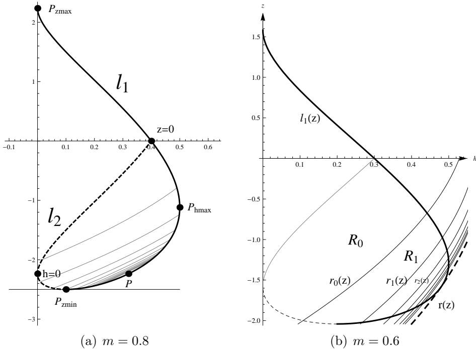
Figure 5: l_1 connects the points P_{zmin} and P_{zmax} , l_2 connects the points P_{zmin} and z = 0
