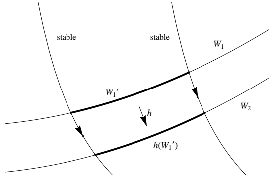
Figure 14: Sliding along stable manifolds
