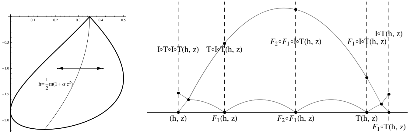
(a) I as a reflection on the phase space
